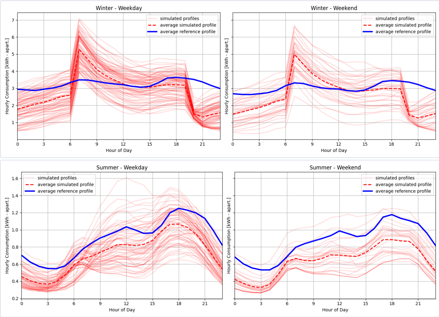
Daily consumption profiles for summer and winter comparing simulated hourly energy use with the reference data. Red lines represent individual days from the model for the given period, the red dashed line indicates the average simulated profile, and the blue line shows the average profile of the reference data. The figures on the left represent weekdays, while the figures on the right represents weekends.
